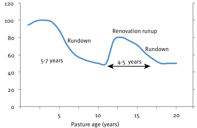
Figure 2: The run-down and run-up of pasture growth over time in response to the repeated use of a blade plough or cutter bar following initial establishment— note the declining level and duration of pasture response over time 1
